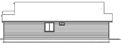
LEFT ELEVATION
