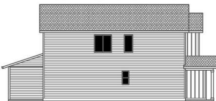
LEFT SIDE ELEVATION SCALE 1/8"=1'-0"
